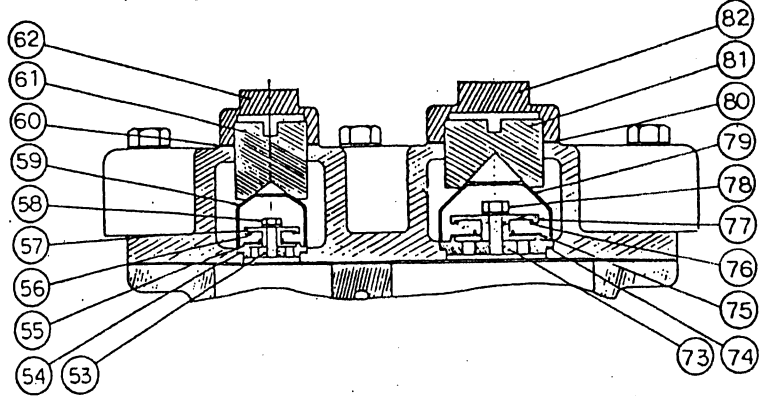
(2段) 吐出弁 (Two Stage) Discharge Valve
